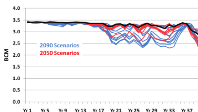
Figure 3-6: Total annual water storage in the Roseries, Senar, Girba, and Jebel Aulia reservoirs under the 2% Growth scenario
