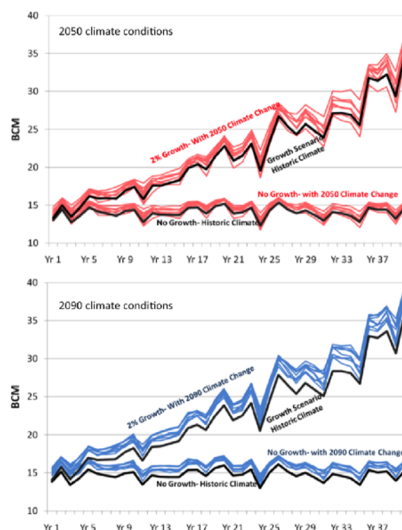
Figure 3-4: Total annual water demands under climate change conditions, 2% Growth and No Growth scenarios
